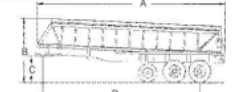
Model OLB326
