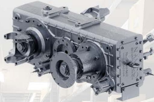
NAMCO 174-C TRANSFER CASE
