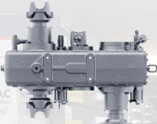
NAMCO 174-C TRANSFER CASE
